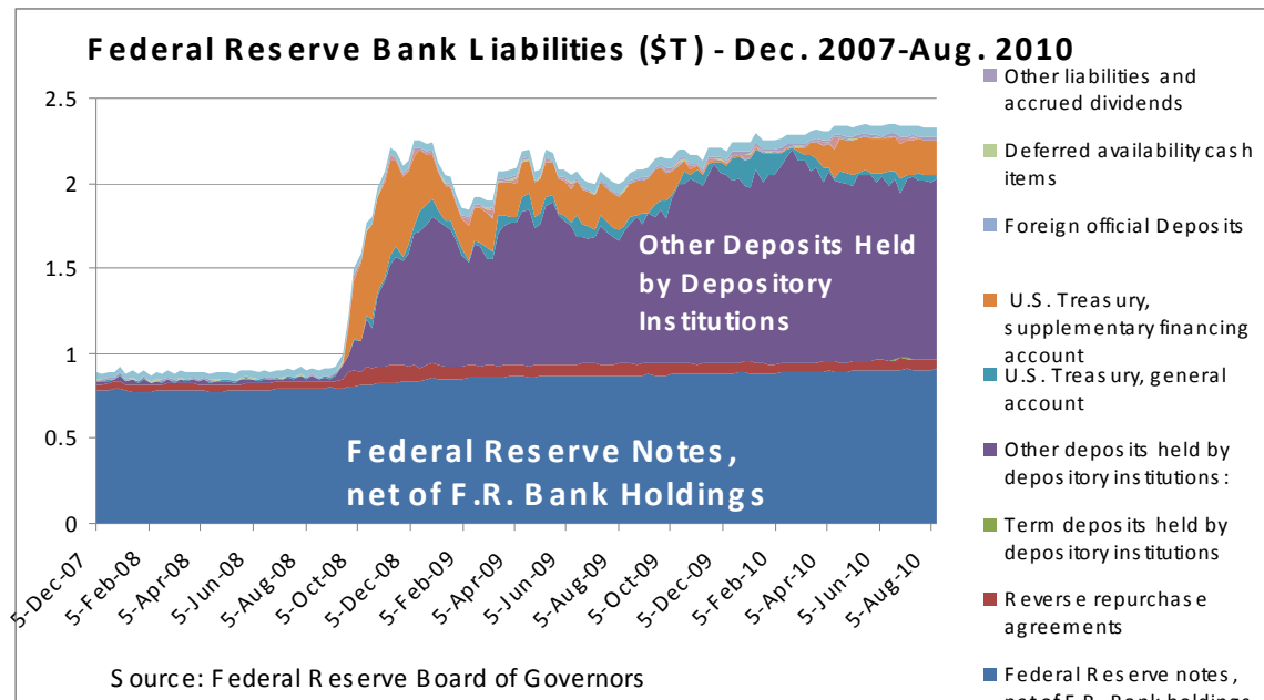
Figure 9: Fed's Liabilities
