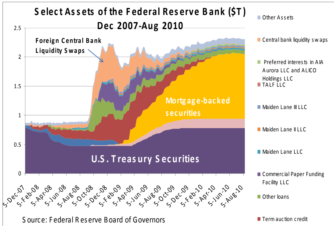
Figure 10: Fed's Assets
